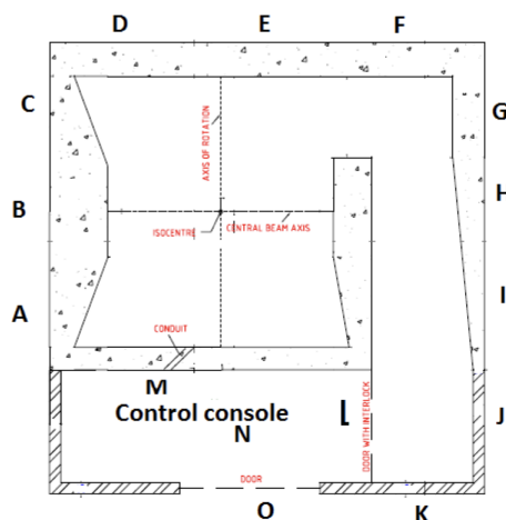
Figure 4: Layout of teletherapy unit in treatment room
